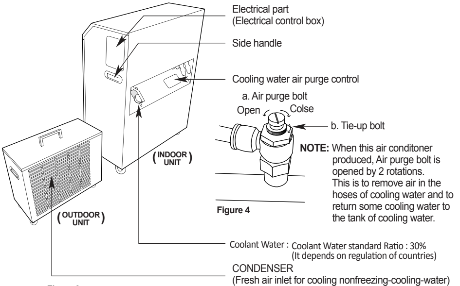
Figure 3 Back and Right Side View
